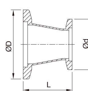
Conical Reducer
