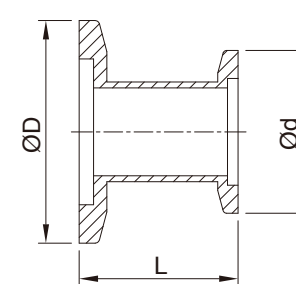
Straight Reducer
